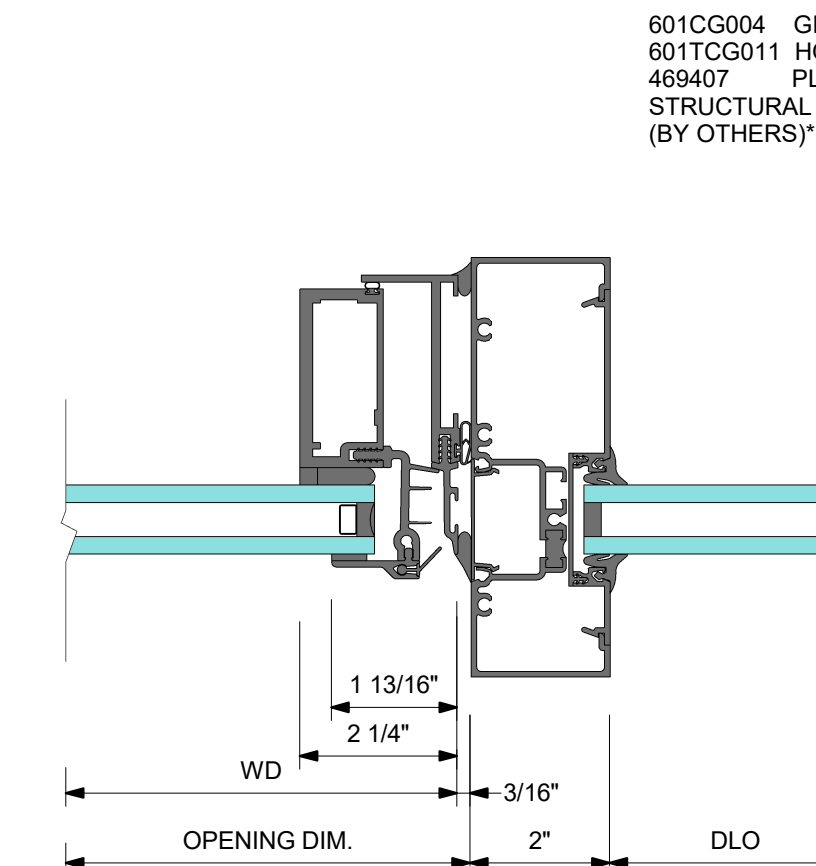
4 VENT @ LEFT
