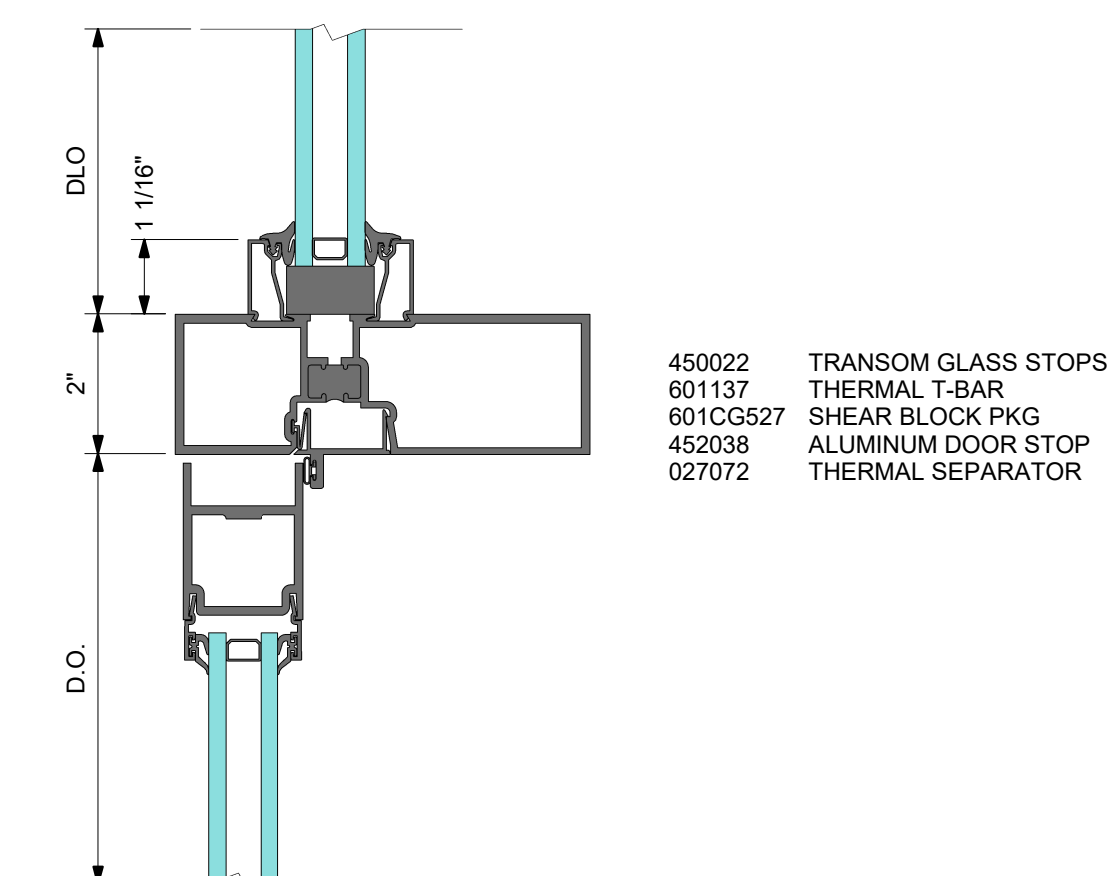
2 DETAIL 2 TRANSOM BAR WITH SURFACE CLOSER
