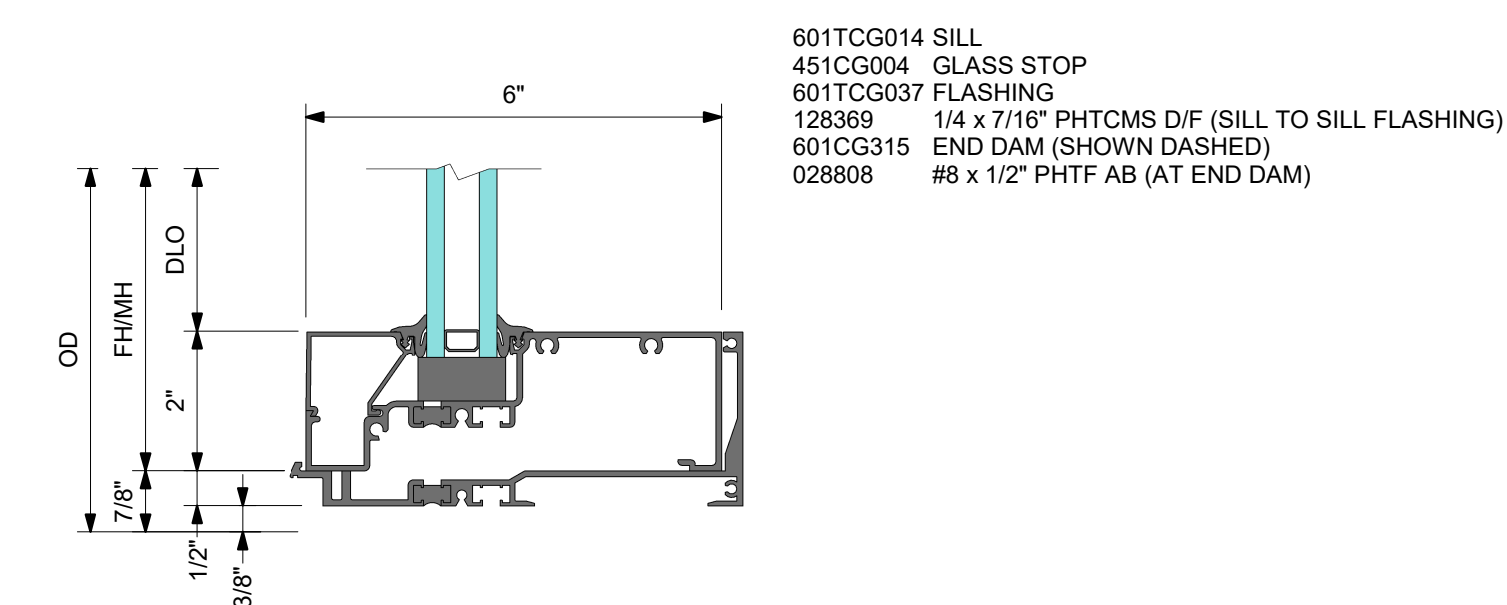
3 DETAIL 3 SILL
