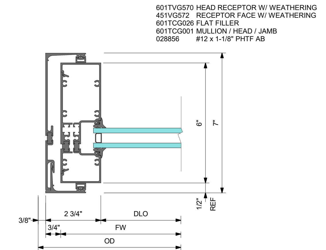
4 DETAIL 4 JAMB WITH RECEPTOR
