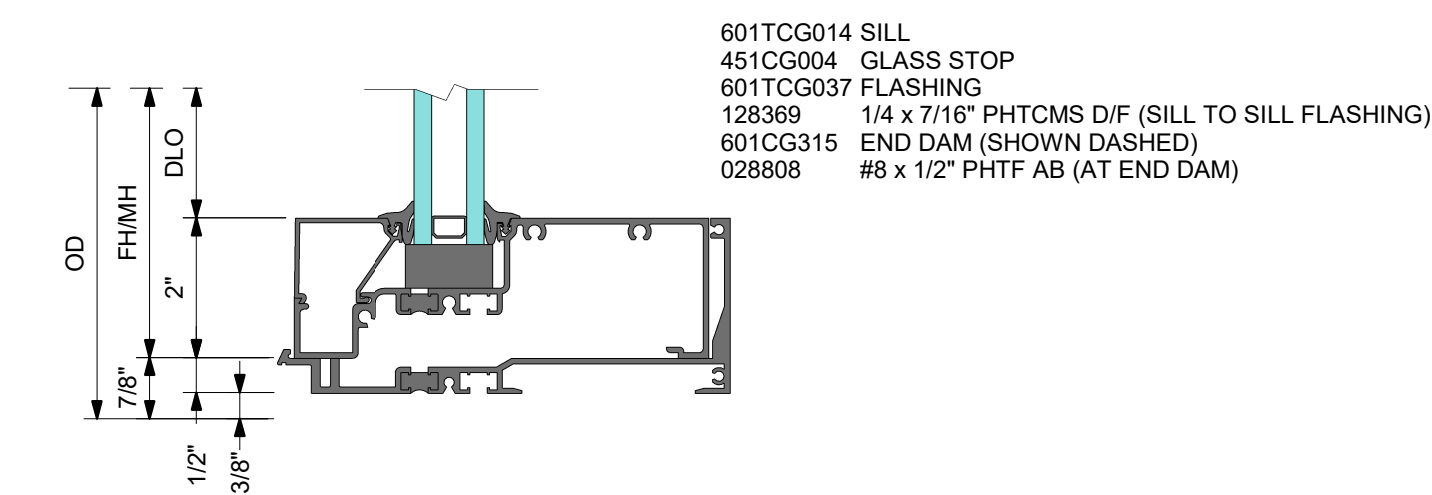
3 DETAIL 3 SILL
