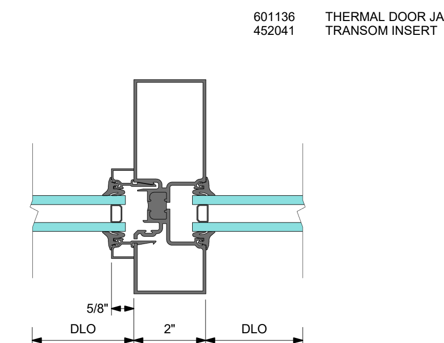
5A DETAIL 5A TRANSOM JAMB WITH SIDELITE
