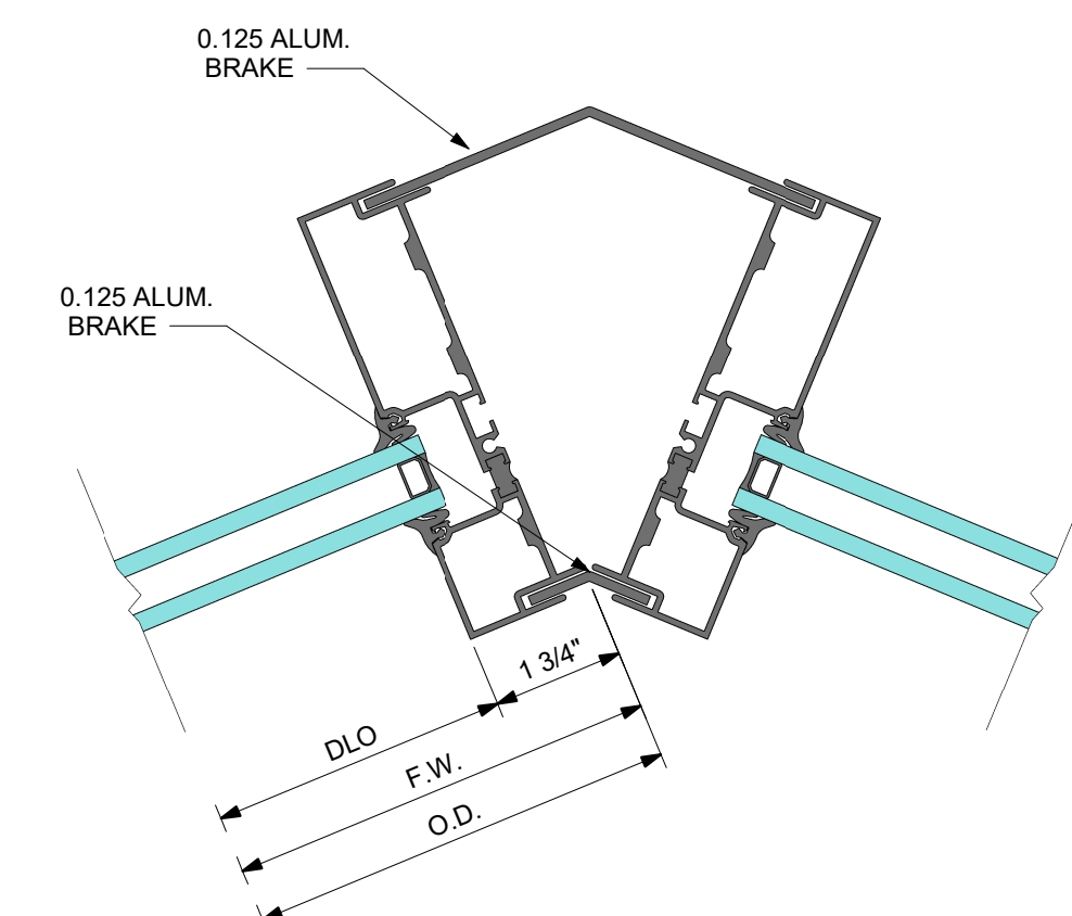
135° INSIDE CORNER WITH BRAKE METAL
