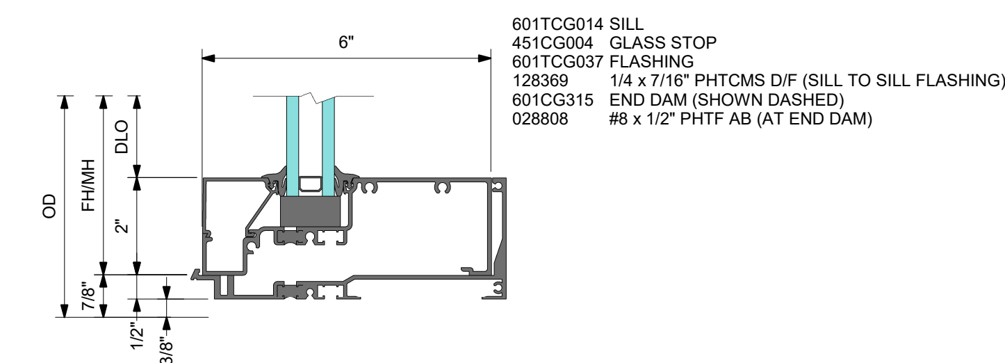
3 DETAIL 3 SILL
