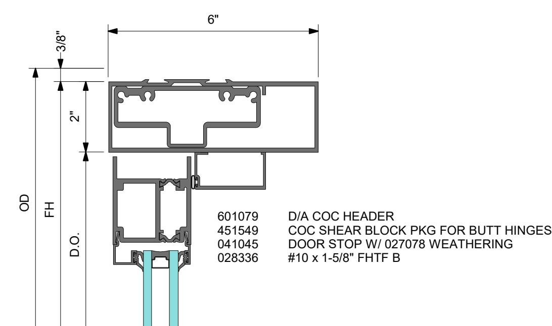
DOOR HEADER WITH KAWNEER CONCEALED CLOSER AND BUTT HINGES
