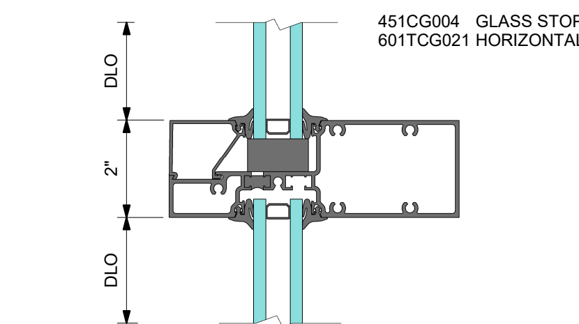
2 DETAIL 2 HORIZONTAL
