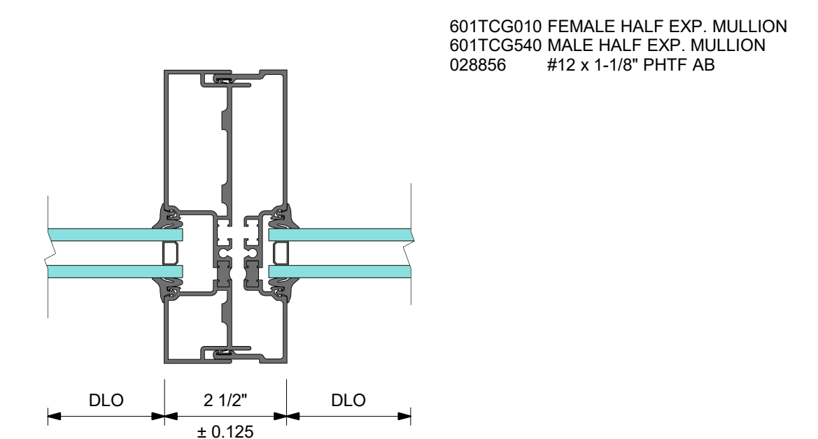
6 DETAIL 6 EXPANSION MULLION
