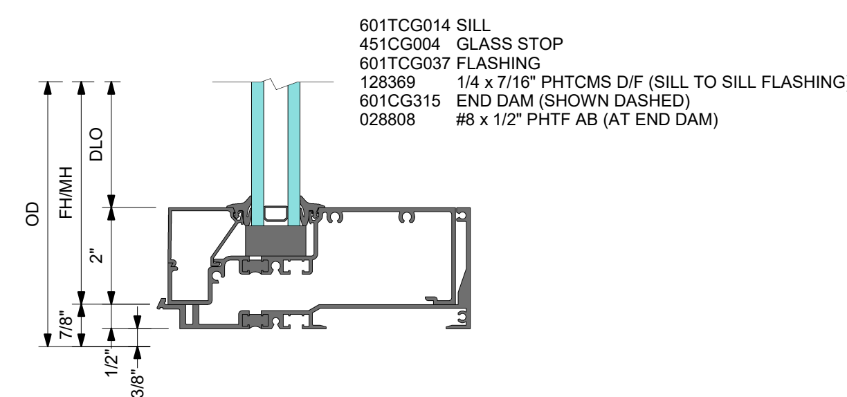
3 DETAIL 3 SILL
