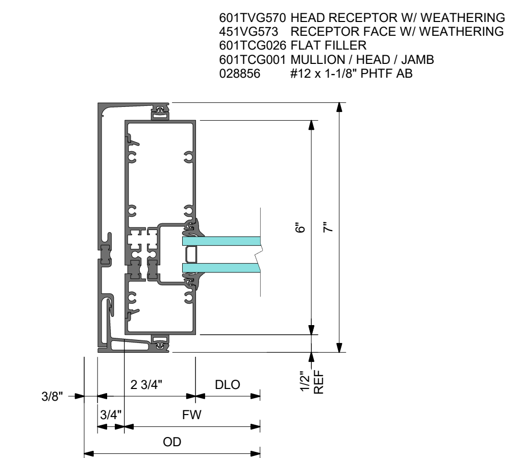
4 DETAIL 4 JAMB WITH HD RECEPTOR
