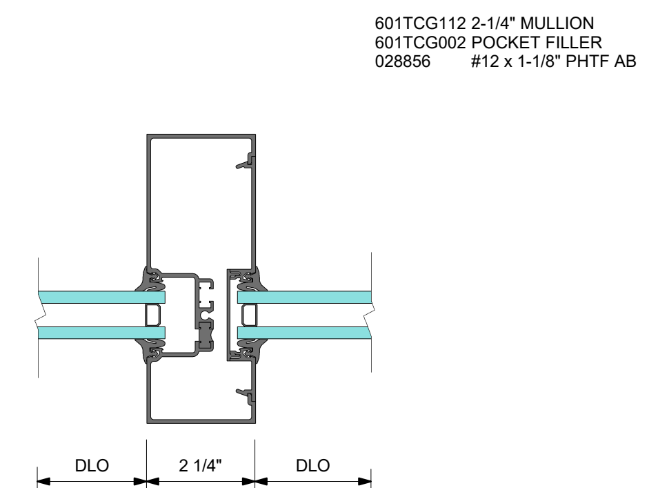
6 DETAIL 6 - 2-1/4" VERTICAL MULLION
