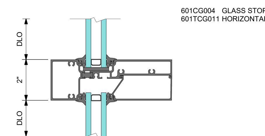
2 DETAIL 2 HORIZONTAL
