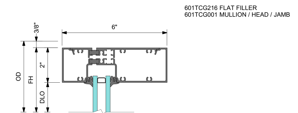
1 DETAIL 1 TRANSOM HEAD
