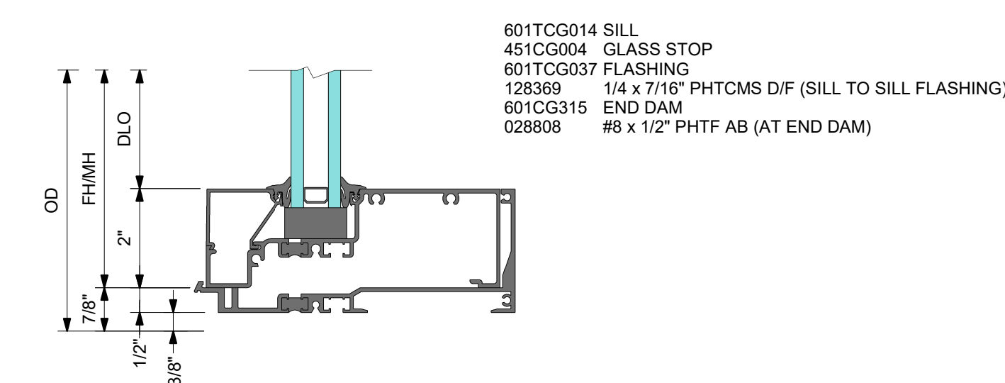
3 DETAIL 3 SILL
