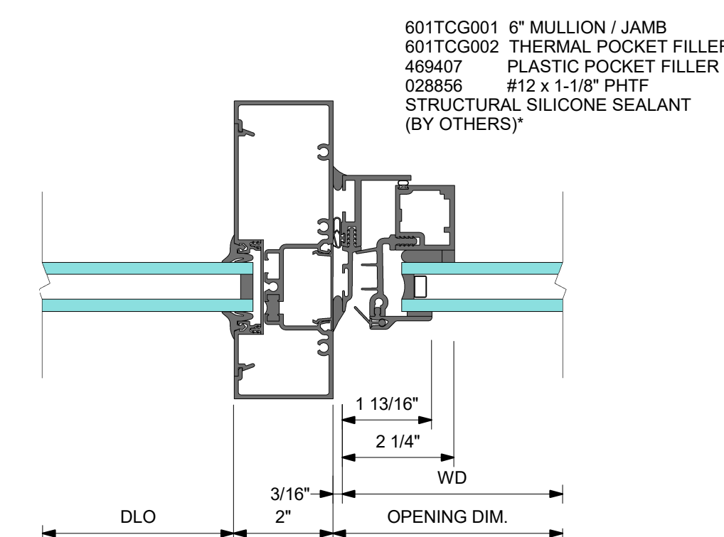
3 VENT @ RIGHT
