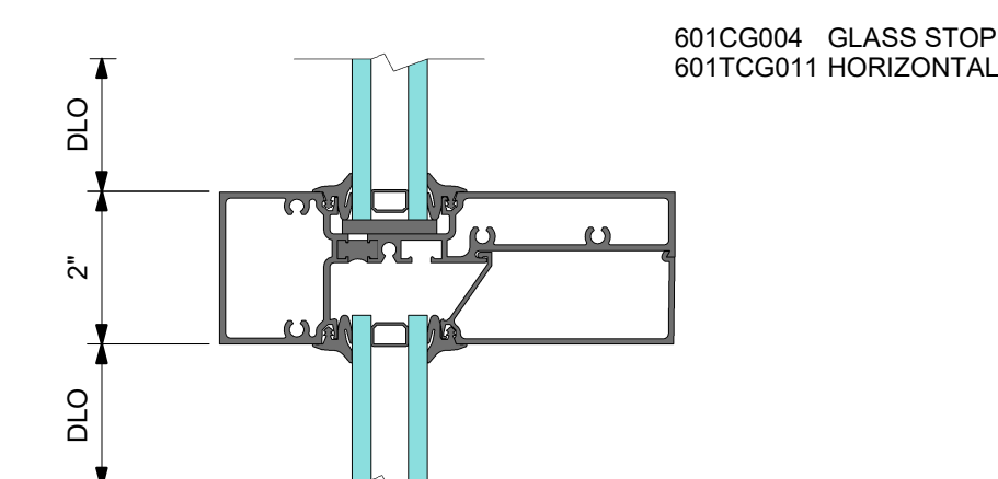
2 DETAIL 2 HORIZONTAL
