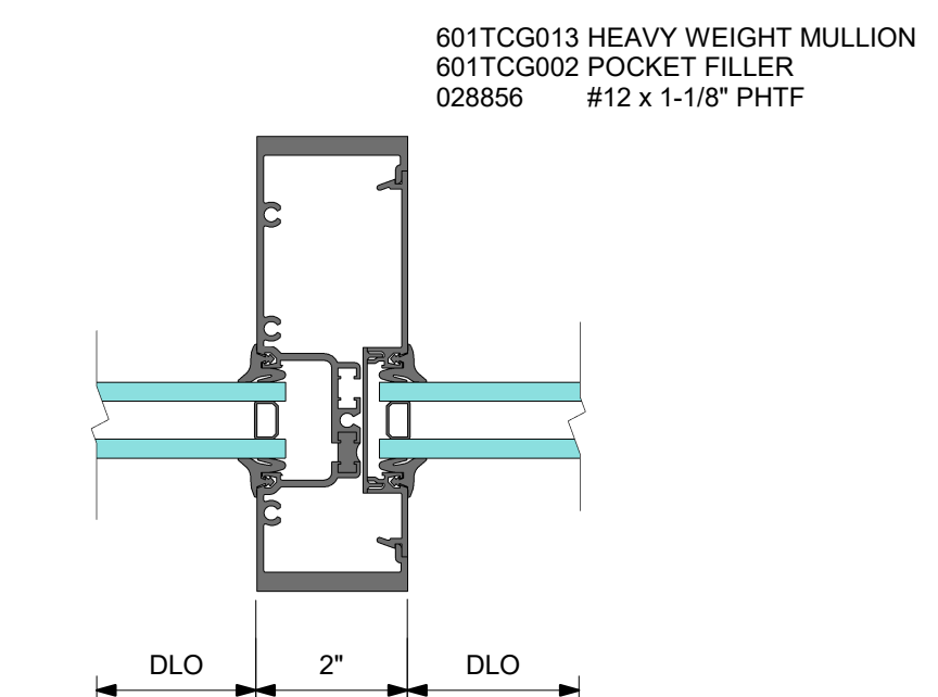
5 DETAIL 5 HEAVY WEIGHT VERTICAL MULLION
