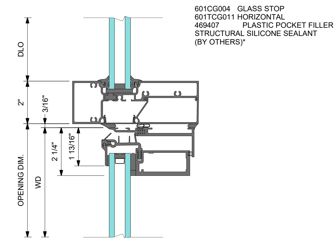
1 VENT HEAD
