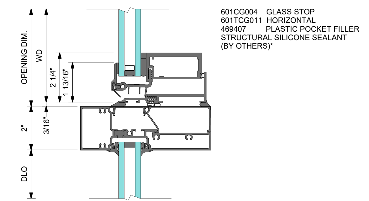
2 VENT SILL
