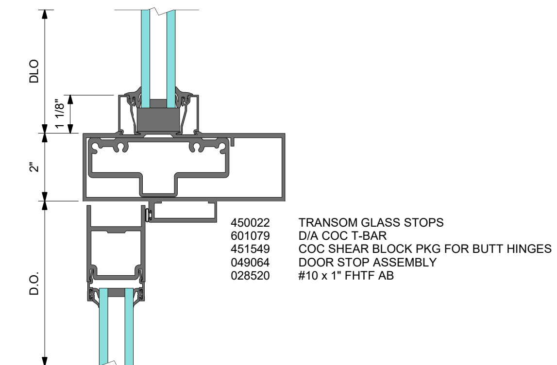
DOOR TRANSOM BAR WITH LCN CONCEALED CLOSER AND OFFSET PIVOTS
