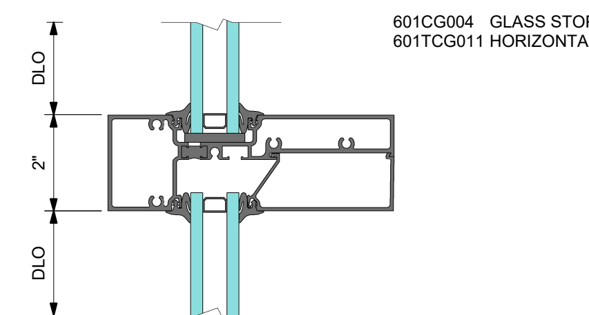
2 DETAIL 2 HORIZONTAL
