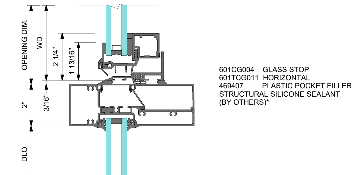
2 VENT SILL
