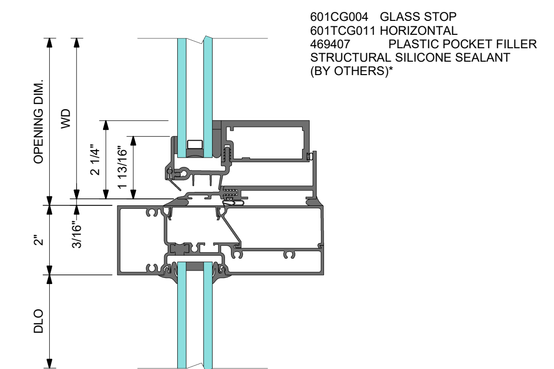
2 VENT SILL
