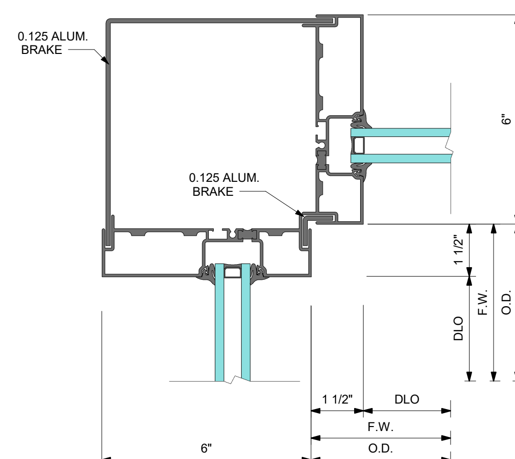
90 INSIDE CORNER WITH BRAKE METAL
