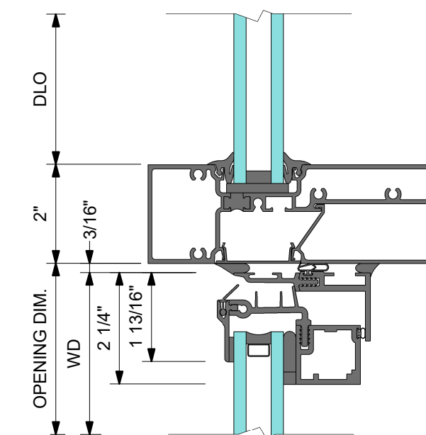
1 VENT HEAD
