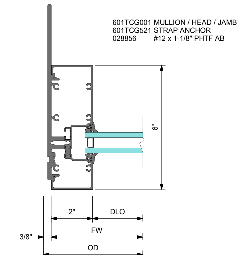
4 DETAIL 4 JAMB WITH STRAP ANCHOR
