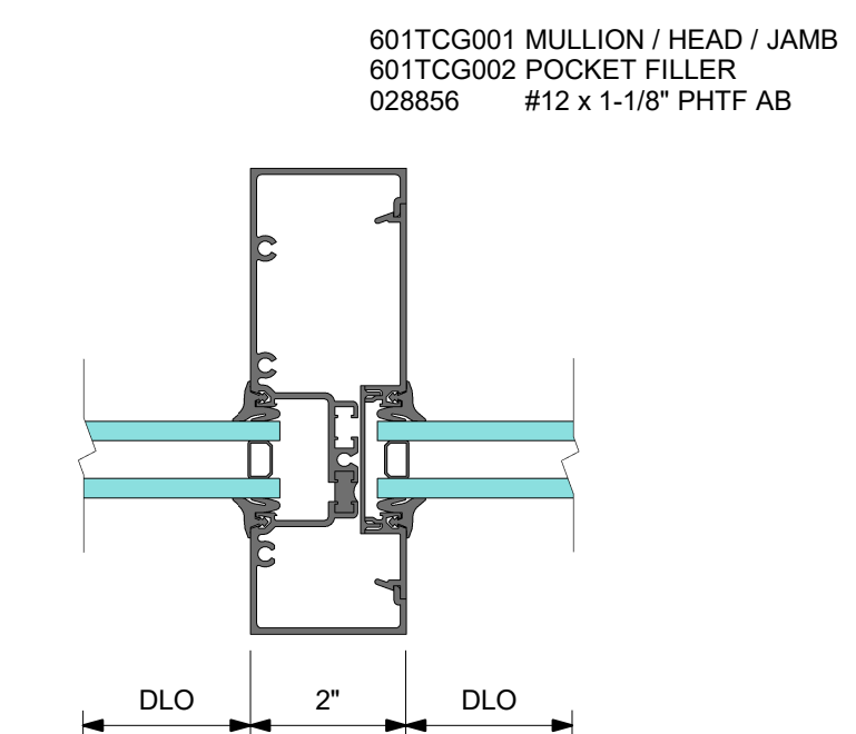
5 DETAIL 5 VERTICAL MULLION
