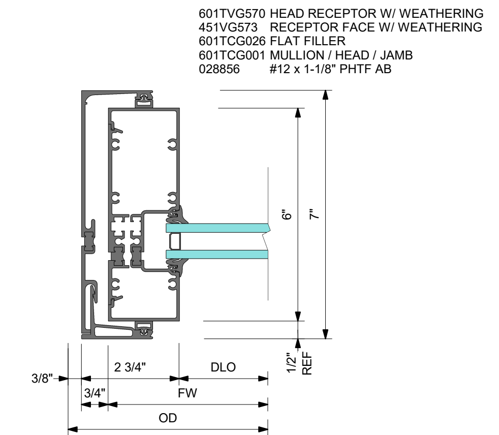
4 DETAIL 4 JAMB WITH HD RECEPTOR
