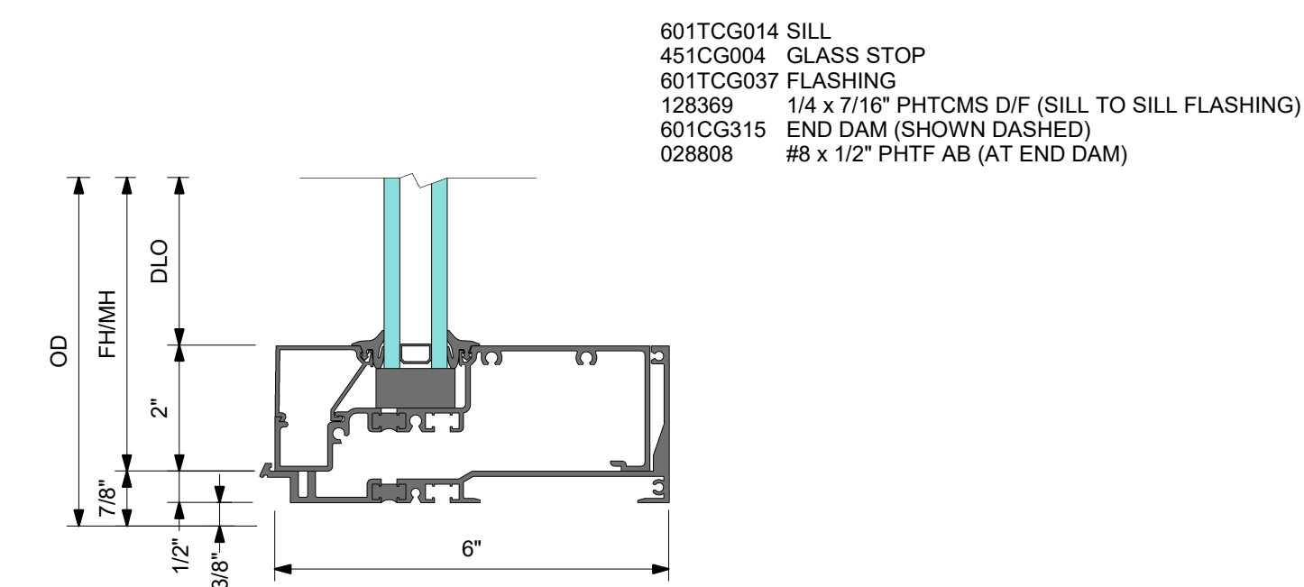
3 DETAIL 3 SILL
