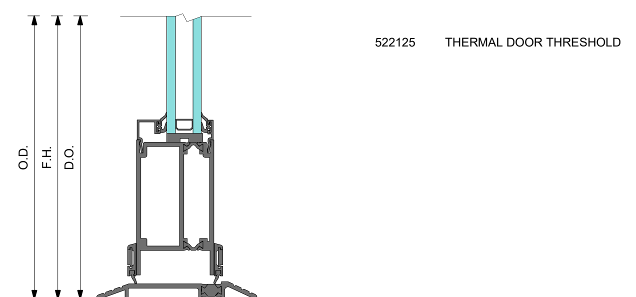
3 DETAIL 3 THRESHOLD
