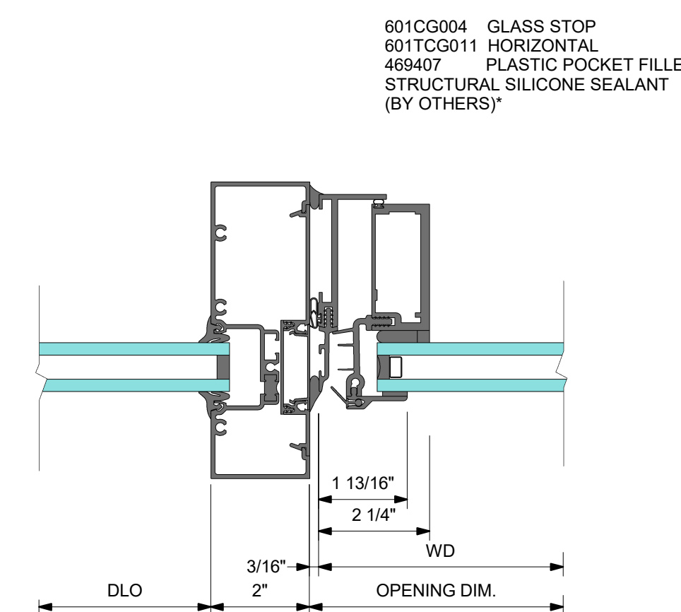
3 VENT @ RIGHT
