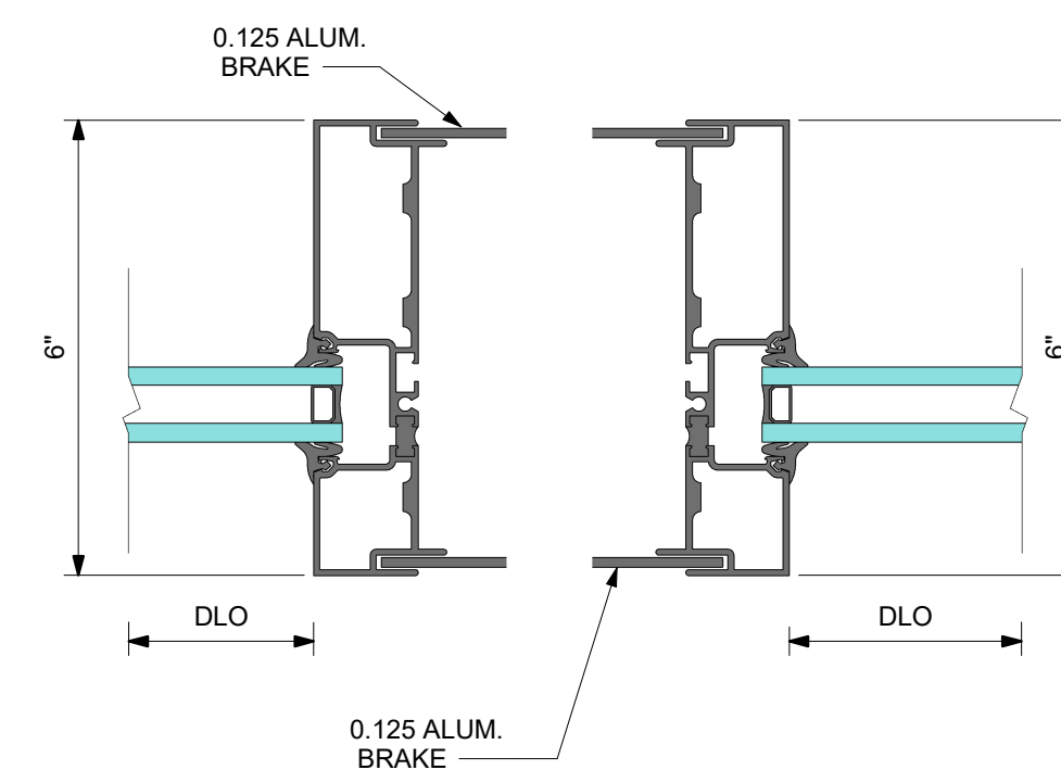
601TCG010 FEMALE EXPANSION MULLION HALF
