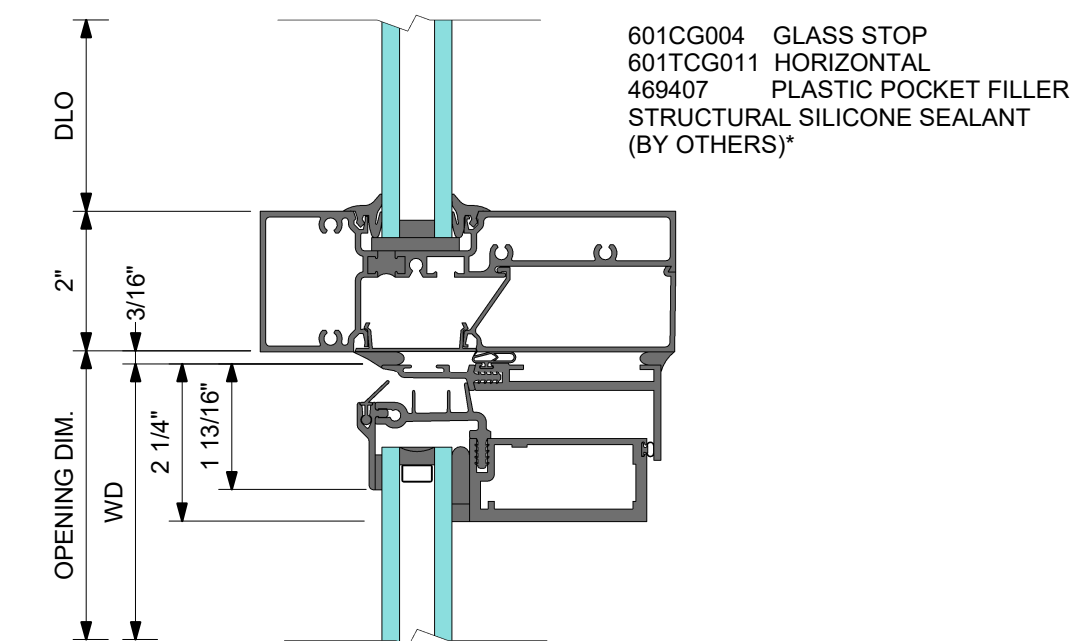
1 VENT HEAD
