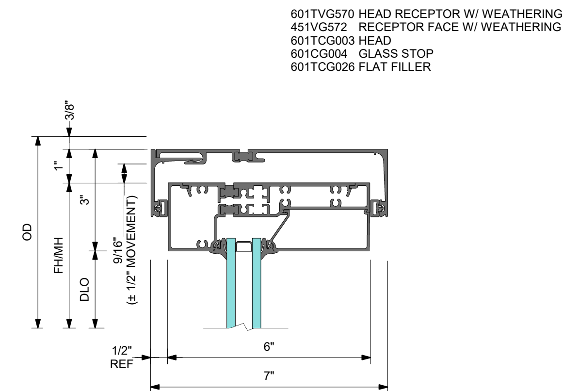
1 DETAIL 1 HEAD WITH RECEPTOR
