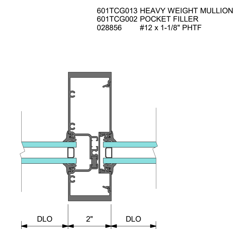
5 DETAIL 5 HEAVY WEIGHT VERTICAL MULLION
