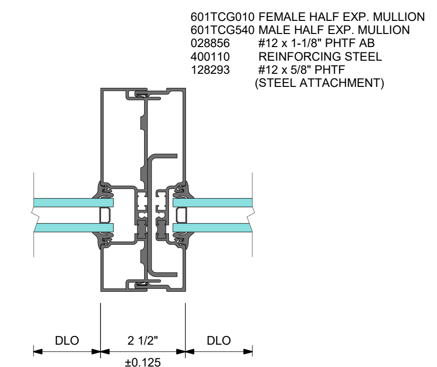
5 DETAIL 5 EXPANSION MULLION WITH STEEL
