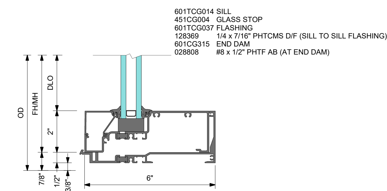
3 DETAIL 3 SILL
