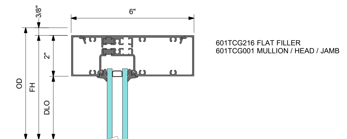
1 DETAIL 1 TRANSOM HEAD
