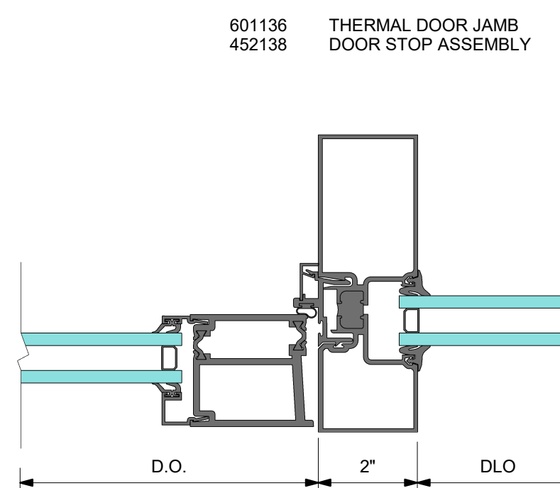
5 DETAIL 5 DOOR JAMB WITH SIDELITE
