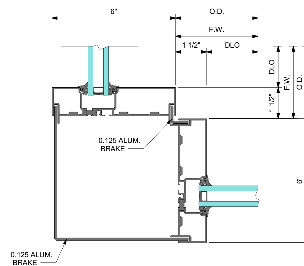
90 OUTSIDE CORNER WITH BRAKE METAL
