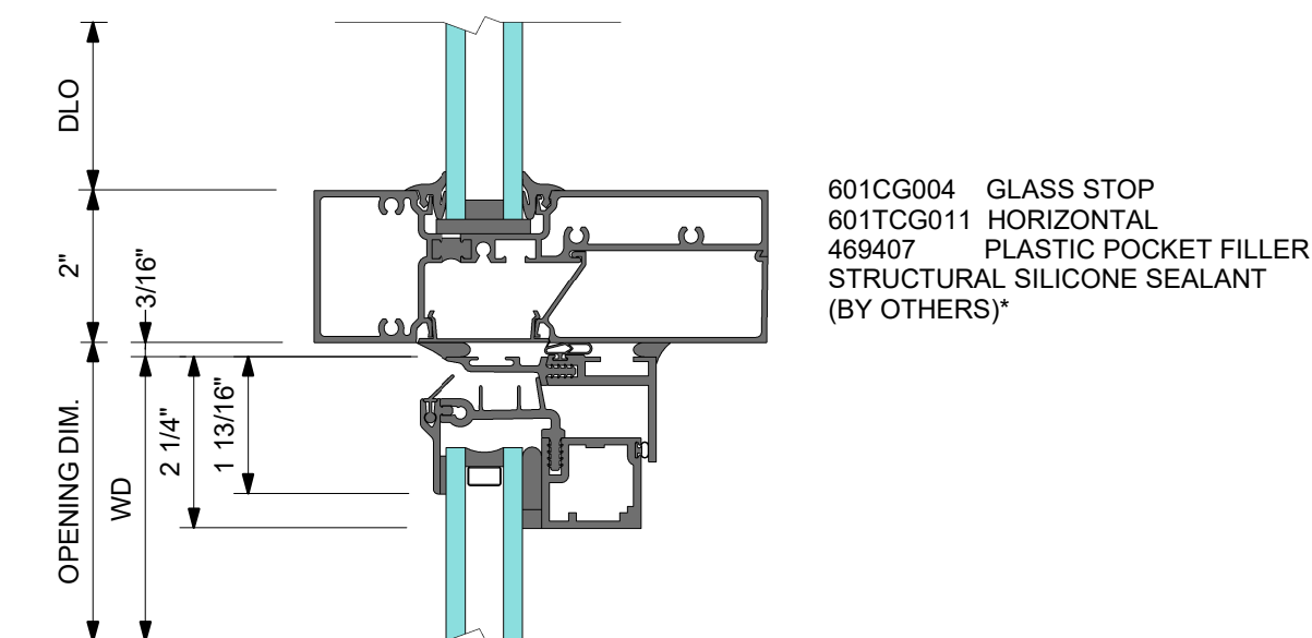
1 VENT HEAD
