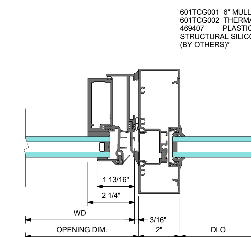
4 VENT @ LEFT
