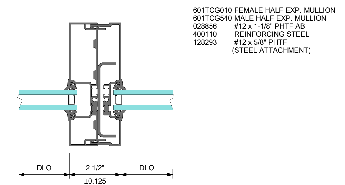
5 DETAIL 5 EXPANSION MULLION WITH STEEL
