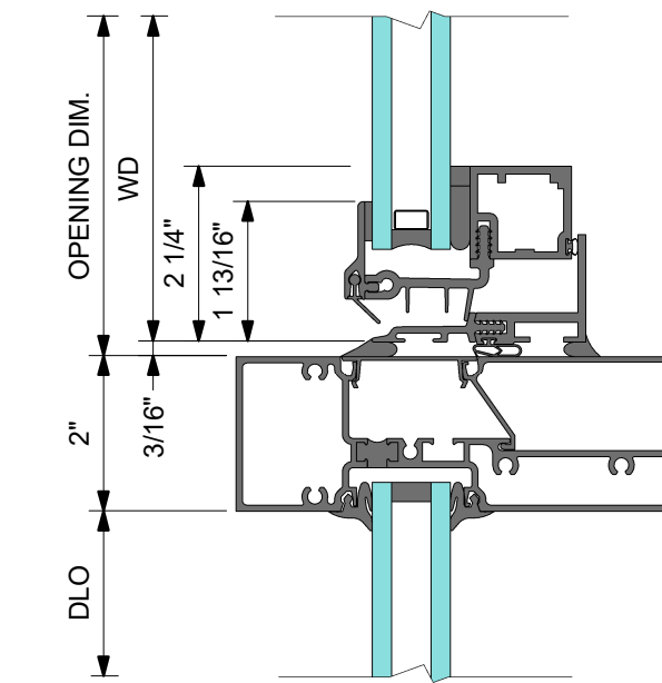
2 VENT SILL
