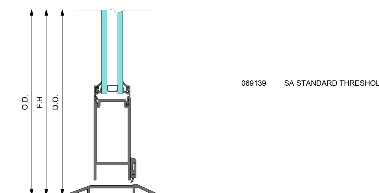
3 DETAIL 3 THRESHOLD
