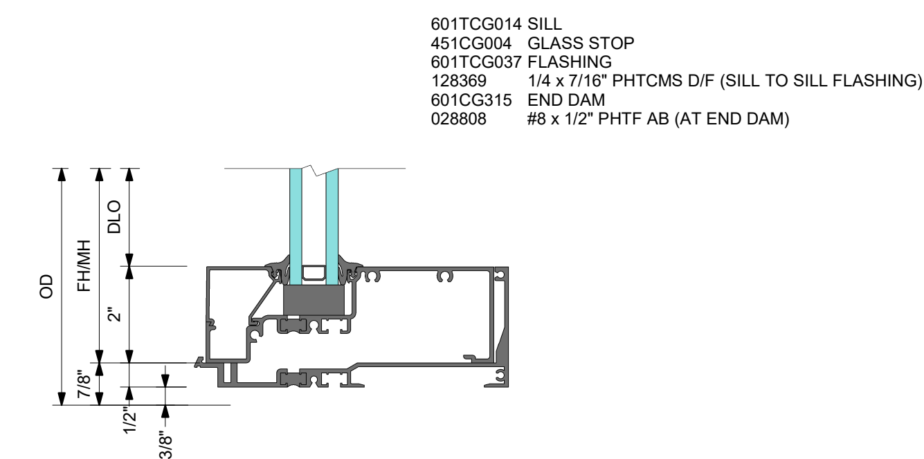
3 DETAIL 3 SILL
