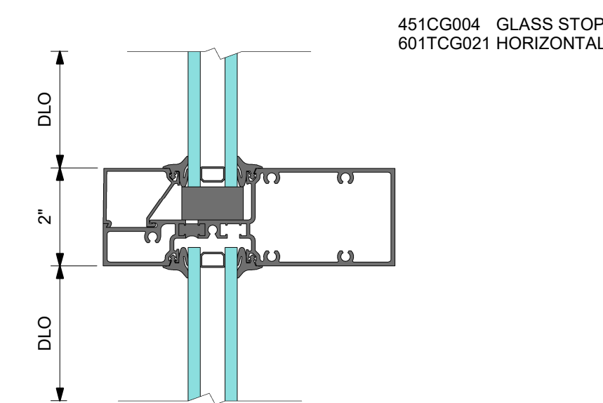
2 DETAIL 2 HORIZONTAL
