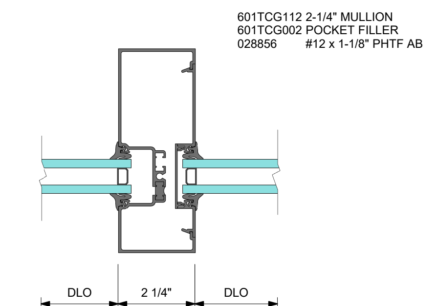
6 DETAIL 6 - 2-1/4" VERTICAL MULLION
