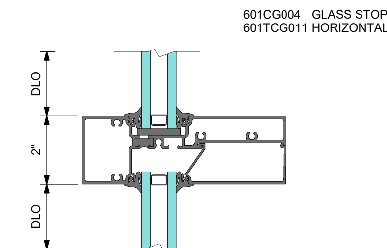
2 DETAIL 2 HORIZONTAL
