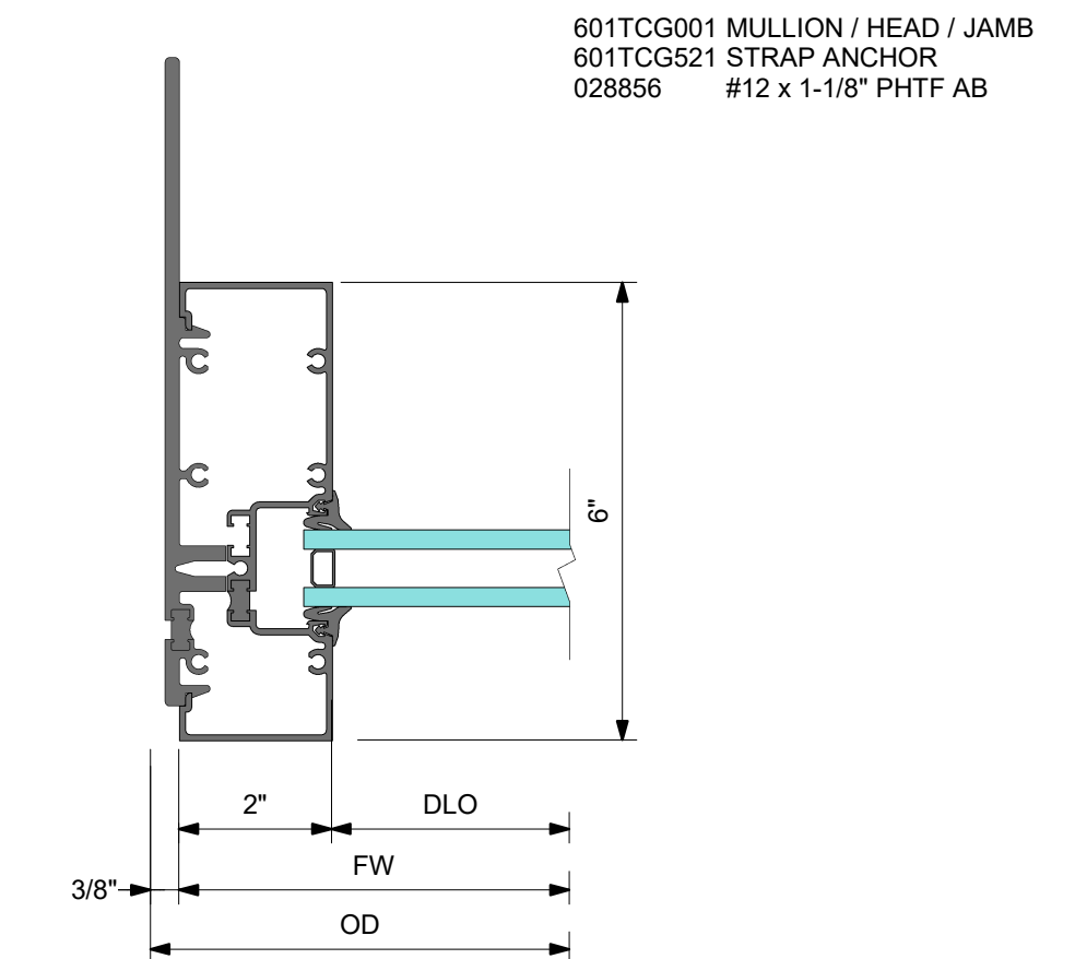
4 DETAIL 4 JAMB WITH STRAP ANCHOR
